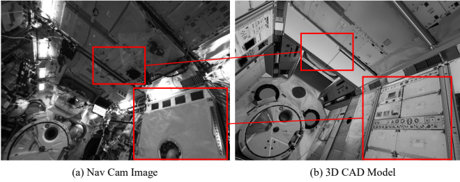
Fig. 12. The mismatched regions (marked by boxes) between the ISS digital twin 3D CAD model and the real environment prevent correct line feature matching, which ultimately limits the effectiveness of our proposed method.
